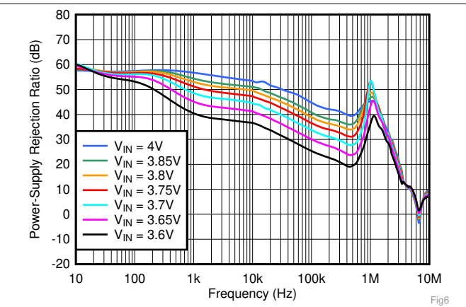
Figure 4. PSRR vs Frequency and V_{IN}
