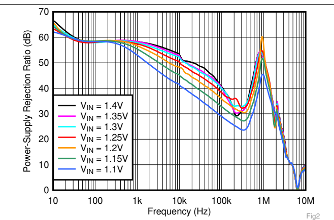
Figure 2. PSRR vs Frequency and V_{IN} With Bias
