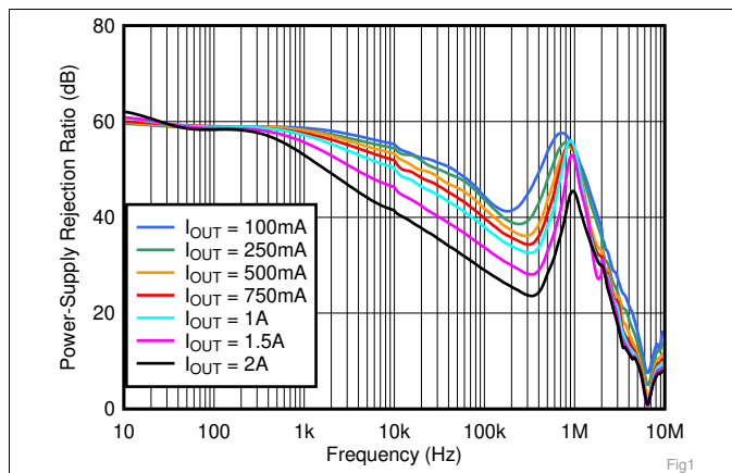
Figure 1. PSRR vs Frequency and I_{OUT}
