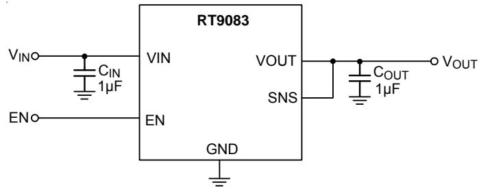
Figure 1. Application with Sense Function
