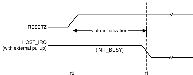
Figure 7-8. HOST_IRQ Timing
