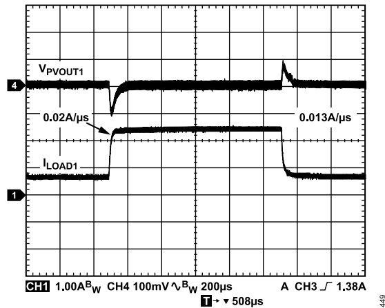
Figure 48. 0.6 A to 2.4 A Load Transient for 2.5 V Output, f_{SW} = 600 kHz, L = 2.2 \mu H, R_C = 1.74 k \Omega , C_C = 22 nF, C_{CP} = 22 pF, C_{PVOUT1} = 47 \mu F
