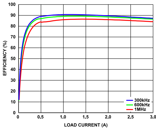
Figure 5. Buck Efficiency vs. Load Current, V_{PVIN1} = 12\text{ V} , V_{PVOUT1} = 3.3\text{ V} at Various Buck Switching Frequencies
