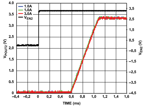
Figure 41. LDO Startup
