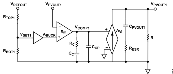
Figure 46. Simplified Peak Current Mode Control, Small Signal Circuit
