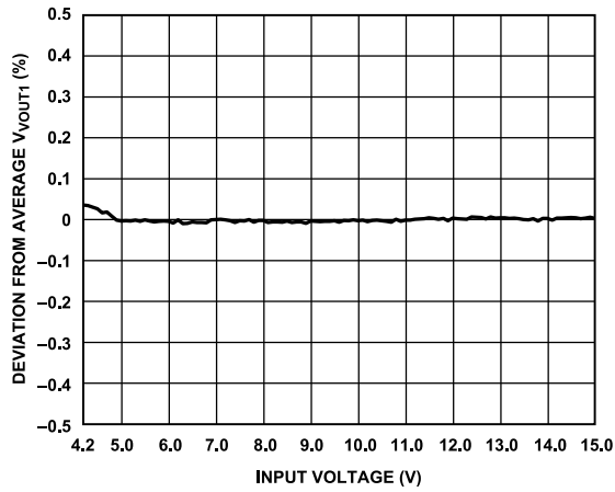
Figure 16. Buck Line Regulation, V_{PVOUT1} = 3.3\text{ V} , I_{LOAD1} = 1\text{ A} , f_{SW} = 600\text{ kHz}
