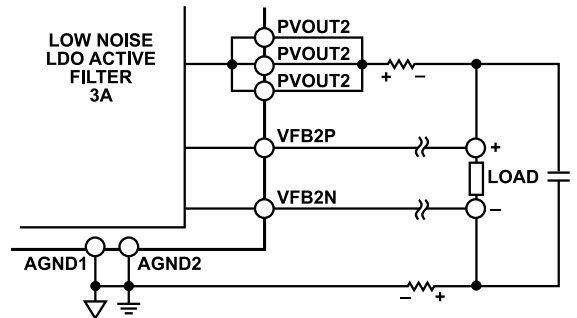
Figure 42. Differential Remote Sensing
