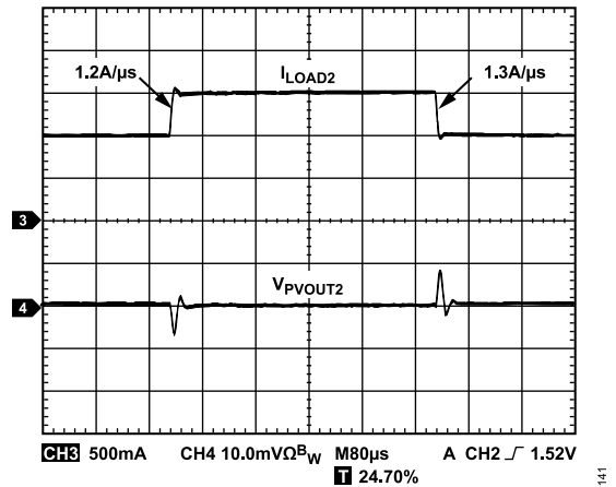
Figure 37. Adaptive Mode Load Transient, V_{PVIN1} = 12\text{ V} , V_{PVOUT2} = 3.3\text{ V} , I_{LOAD2} = 1\text{ A to }1.5\text{ A} , f_{SW} = 1.5\text{ MHz} , L = 2.2\text{ }\mu\text{H} , R_C = 3.48\text{ k}\Omega , C_C = 22\text{ nF} , C_{CP} = 22\text{ pF} , C_{PVOUT1} = 64\text{ }\mu\text{F}
