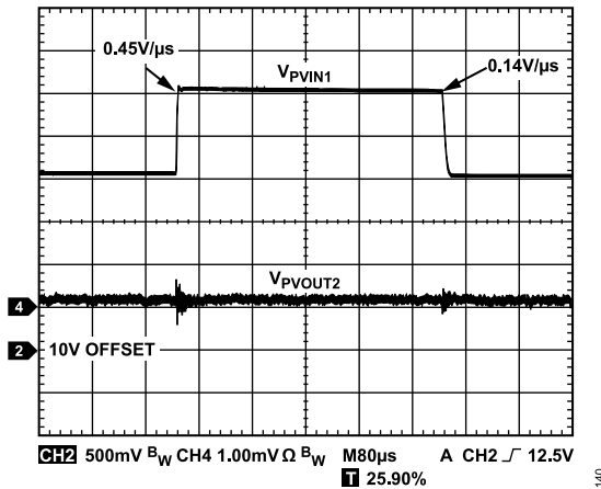
Figure 34. Adaptive Mode Line Transient, V_{PVIN1} = 11\text{ V to }13\text{ V} , V_{PVOUT2} = 3.3\text{ V} , I_{LOAD2} = 1\text{ A} , f_{SW} = 1.5\text{ MHz} , L = 2.2\text{ }\mu\text{H} , R_C = 3.48\text{ k}\Omega , C_C = 22\text{ nF} , C_{CP} = 22\text{ pF} , C_{PVOUT1} = 64\text{ }\mu\text{F}
