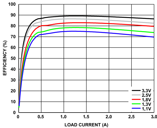
Figure 4. Buck Efficiency vs. Load Current, V_{PVIN1} = 12\text{ V} , f_{SW} = 600\text{ kHz} at Various Buck Output Voltages
