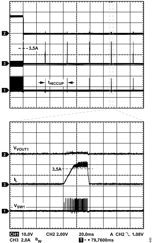
Figure 40. Short-Circuit Response (Current Limit and Hiccup Mode)
