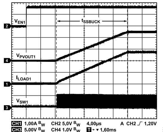
Figure 39. Buck Startup
