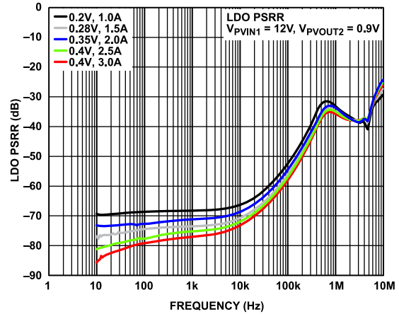
Figure 51. LDO PSRR vs. Frequency
