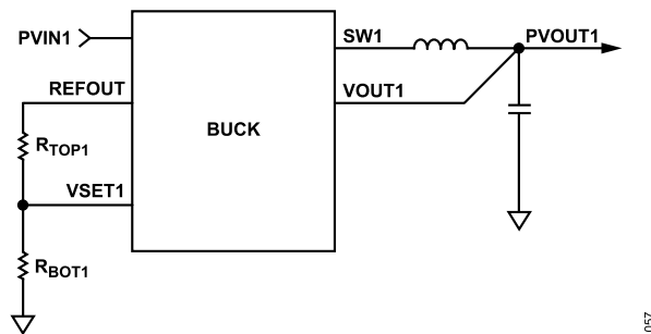
Figure 44. Buck Regulator Adjustable Output Voltage
