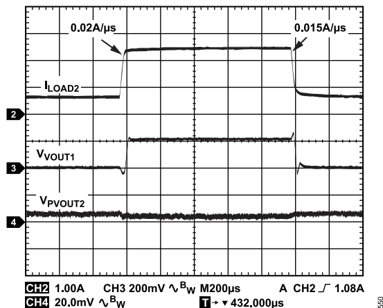
Figure 47. 0.6 A to 2.4 A Load Transient for 2.5 V Output, f_{SW} = 0.6 \text{ MHz} , L = 3.3 \mu\text{H} , R_C = 9.76 \text{ k}\Omega , C_C = 4.7 \text{ nF} , C_{CP} = 4.7 \text{ pF} , C_{PVOUT1} = 44 \mu\text{F}
