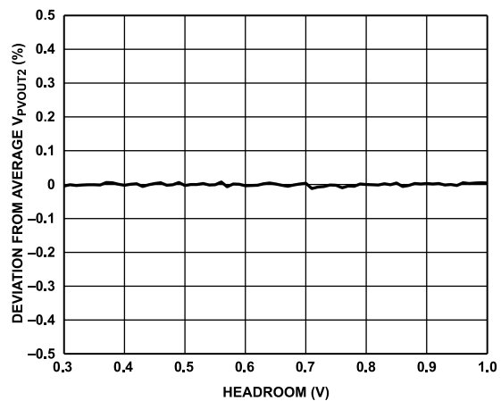
Figure 17. LDO Line Regulation, V_{PVOUT2} = 3.3\text{ V} , I_{LOAD2} = 1\text{ A}
