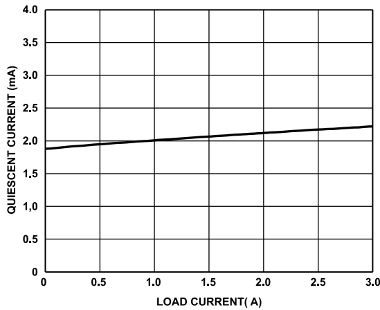
Figure 22. LDO Quiescent Current vs. Load Current
