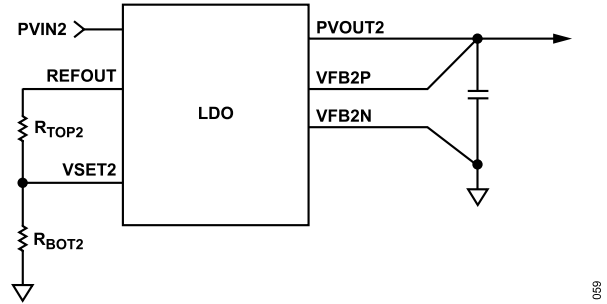
Figure 45. LDO Adjustable Output Voltage Configuration
