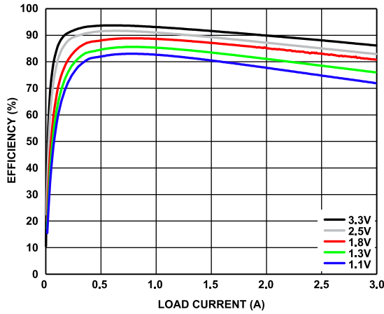
Figure 3. Buck Efficiency vs. Load Current, V_{PVIN1} = 5\text{ V} , f_{SW} = 600\text{ kHz} at Various Buck Output Voltages
