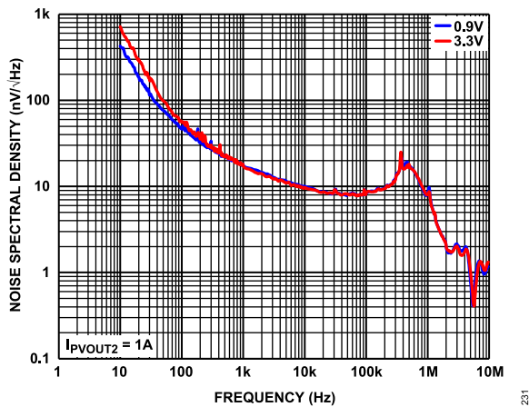
Figure 11. LDO Noise Spectral Density vs. Frequency at Various LDO Output Voltages
