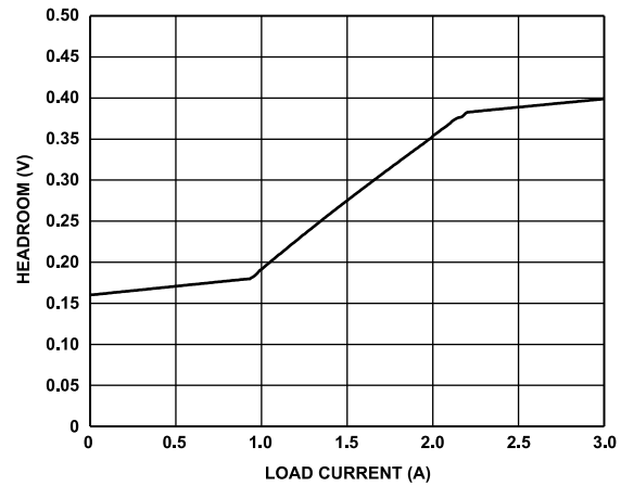
Figure 25. Adaptive Mode Headroom vs. Load Current
