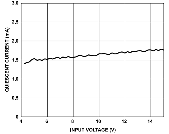
Figure 24. Buck Quiescent Current vs. Input Voltage
