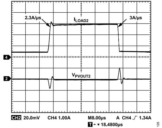
Figure 36. LDO Load Transient, V_{PVIN2} = 3.6\text{ V} , V_{PVOUT2} = 3.3\text{ V} , I_{LOAD2} = 0.5\text{ A to }3\text{ A}
