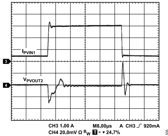
Figure 35. Adaptive Mode Load Transient, V_{PVIN1} = 12\text{ V} , V_{PVOUT2} = 3.3\text{ V} , I_{LOAD2} = 0.5\text{ A to }3\text{ A} , f_{SW} = 1.5\text{ MHz} , L = 2.2\text{ }\mu\text{H} , R_C = 3.48\text{ k}\Omega , C_C = 22\text{ nF} , C_{CP} = 22\text{ pF} , C_{PVOUT1} = 64\text{ }\mu\text{F}
