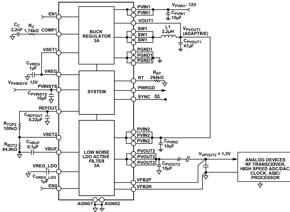
Figure 52. Adaptive Headroom Configuration
