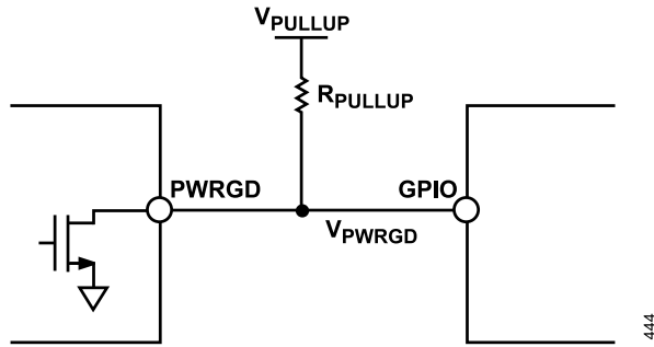
Figure 43. Power-Good Setup
