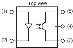
Internal circuit
