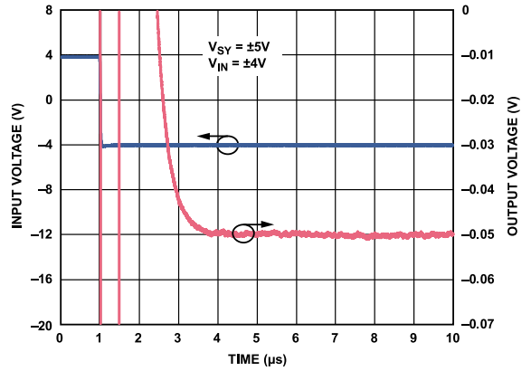
Figure 66. Negative Settling Time, A_V = -10 , V_{SY} = \pm 5 V
