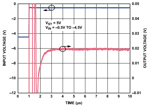
Figure 64. Positive Settling Time, A_V = -10 , V_{SY} = 5 V
