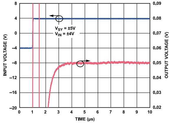
Figure 63. Positive Settling Time, A_V = -10 , V_{SY} = \pm 5 V
