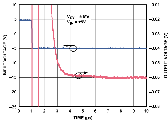
Figure 65. Negative Settling Time, A_V = -10 , V_{SY} = \pm 15 V
