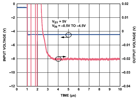
Figure 67. Negative Settling Time, A_V = -10 , V_{SY} = 5 V
