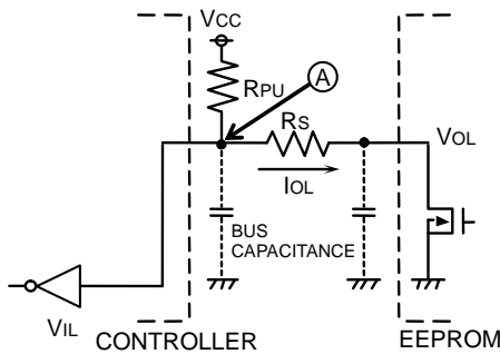
Fig.46 I/O Circuit
