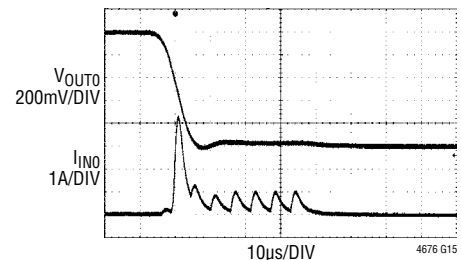
FIGURE 44 CIRCUIT AT 12\text{V}_{\text{IN}} , NO LOAD ON V_{\text{OUT0}} PRIOR TO APPLICATION OF SHORT CIRCUIT
