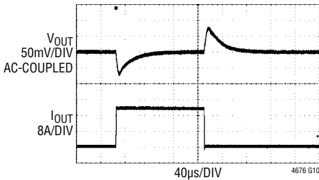
FIGURE 35 CIRCUIT AT 5\text{V}_{\text{IN}} , V_{\text{OUT\_COMMAND}_n} SET TO 1.000V. 0A TO 20A LOAD STEP AT 20A/µs
