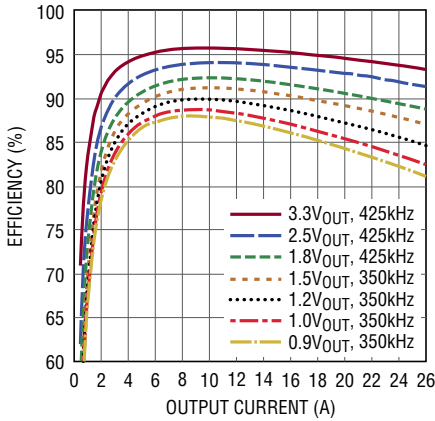
Efficiency vs Output Current, 5V_{IN} , V_{OUT0} and V_{OUT1} Paralleled, V_{IN} = SV_{IN} = V_{INn} = INTV_{CC} , MFR\_PWM\_MODE_n[1:0] = 10_b
