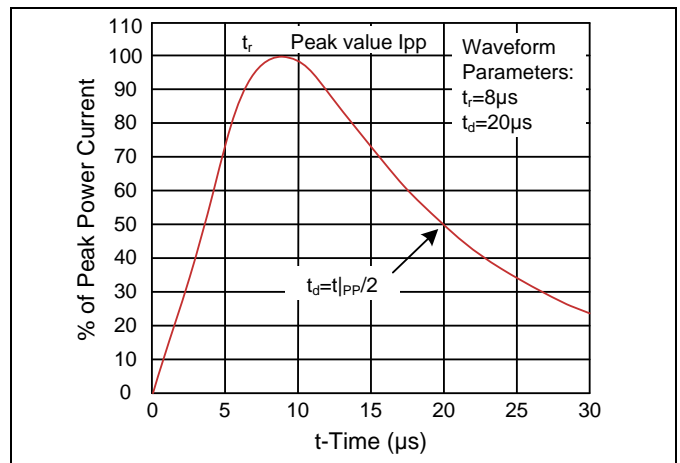
Figure 2. Pulse Waveform
