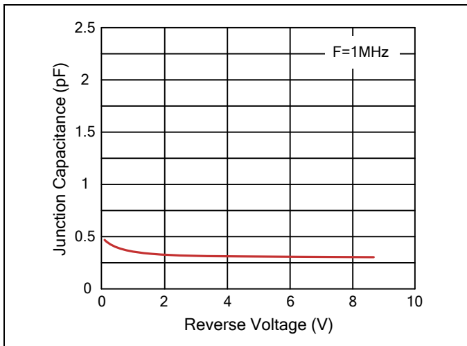
Figure 3. Normalized Capacitance vs. Reverse Voltage
