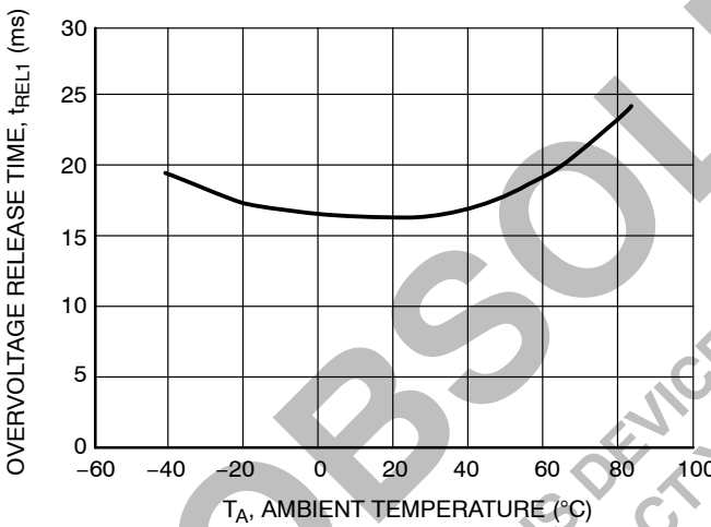
Figure 7. Overvoltage Release Time vs. Temperature
