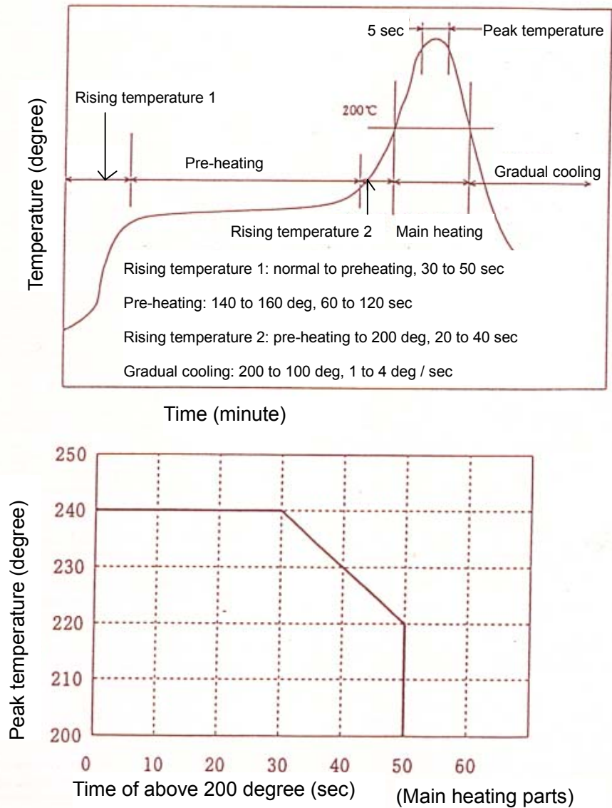
Fig.28. The limit of resistance to soldering heat of surface mount resistor
