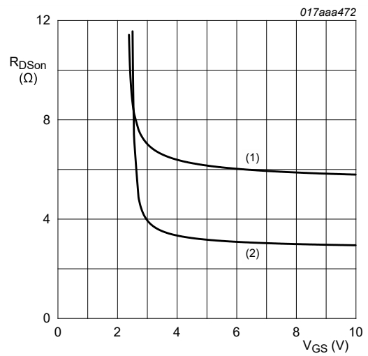
Fig. 9. Drain-source on-state resistance as a function of gate-source voltage; typical values I_D = 0.2\text{ A} (1) T_j = 150\text{ }^\circ\text{C} (2) T_j = 25\text{ }^\circ\text{C}
