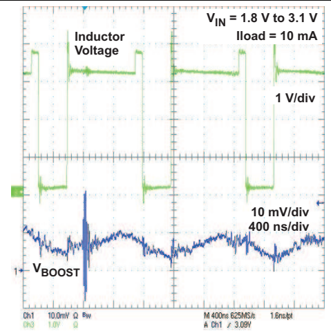
Figure 9. Boost Switching Waveform, Continuous-Current Mode
