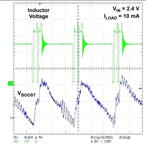
Figure 10. Boost Switching Waveform, Discontinuous-Current Mode
