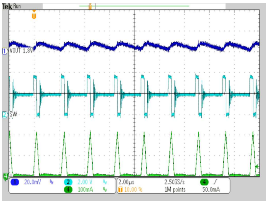
V_{IN} = 3.6\text{ V} I_{OUT} = 25\text{ mA} L = 2.2\text{ }\mu\text{H} C_{OUT} = 10\text{ }\mu\text{F} CTRL = \text{GND}
