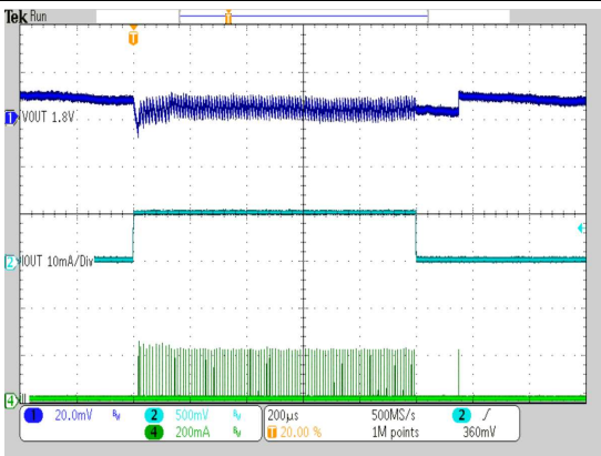
V_{IN} = 3.6\text{ V} I_{OUT} = 50\text{ }\mu\text{A} to 10\text{ mA} L = 2.2\text{ }\mu\text{H} C_{OUT} = 10\text{ }\mu\text{F} CTRL = \text{GND}
