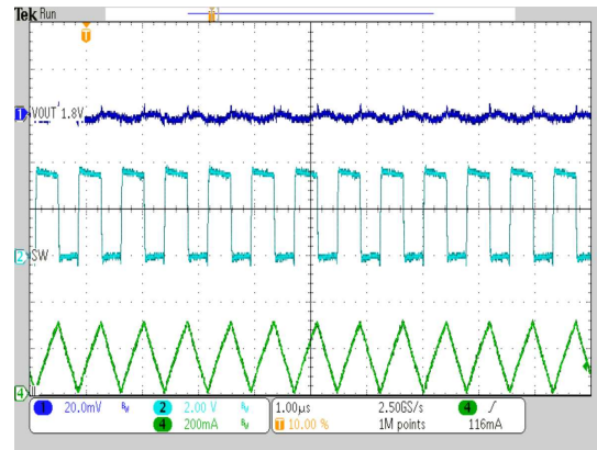
V_{IN} = 3.6\text{ V} I_{OUT} = 150\text{ mA} L = 2.2\text{ }\mu\text{H} C_{OUT} = 10\text{ }\mu\text{F} CTRL = \text{GND}
