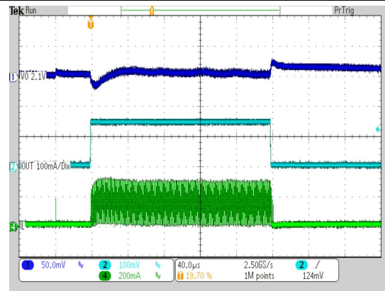
V_{IN} = 3.6\text{ V} I_{OUT} = 0.5\text{ mA} to 150\text{ mA} L = 2.2\text{ }\mu\text{H} C_{OUT} = 10\text{ }\mu\text{F} CTRL = V_{IN}
