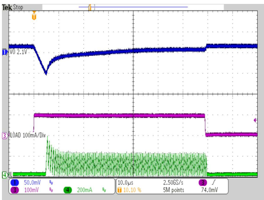
V_{IN} = 3.6\text{ V} , V_{OUT} = 2.1\text{ V} L = 2.2\text{ }\mu\text{H} C_{OUT} = 10\text{ }\mu\text{F} Loadstep at V_{OUT} 0 mA to 100 mA, 1 µs rise/ fall time, 70 µs / 7 ms
