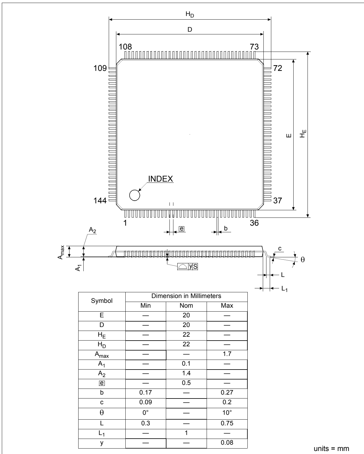
Figure 23-1: SID13743 QFP20 144-pin Package
