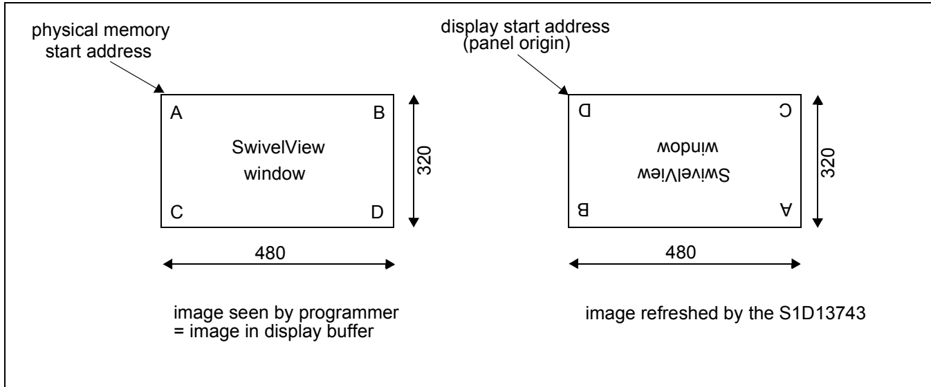
Figure 18-2: Relationship Between The Screen Image and the Image Refreshed in 180° SwivelView
