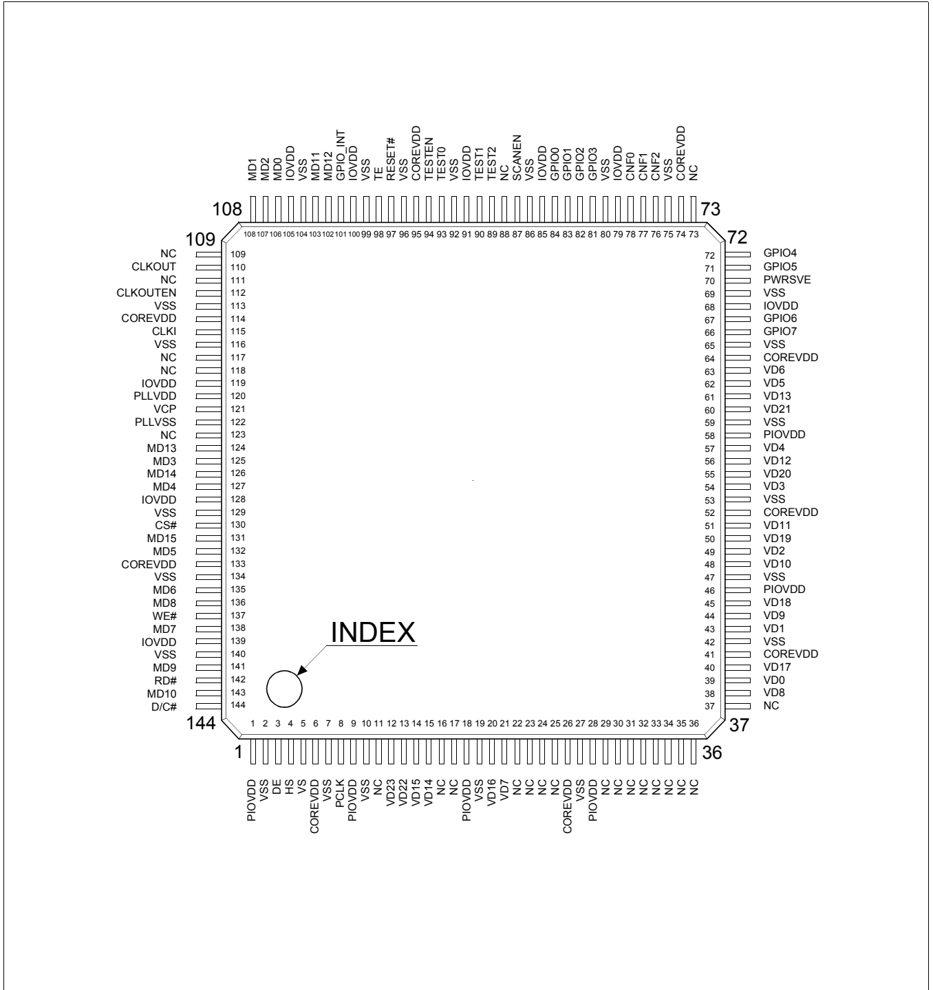
Figure 4-1: SID13743 QFP20 Pinout (Top View)
