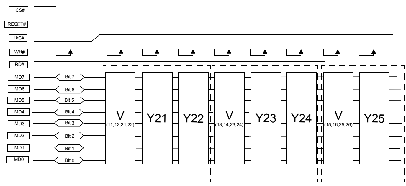
Figure 15-4: YUV 4:2:0 EVEN Line with Intel 80, 8-bit Interface
