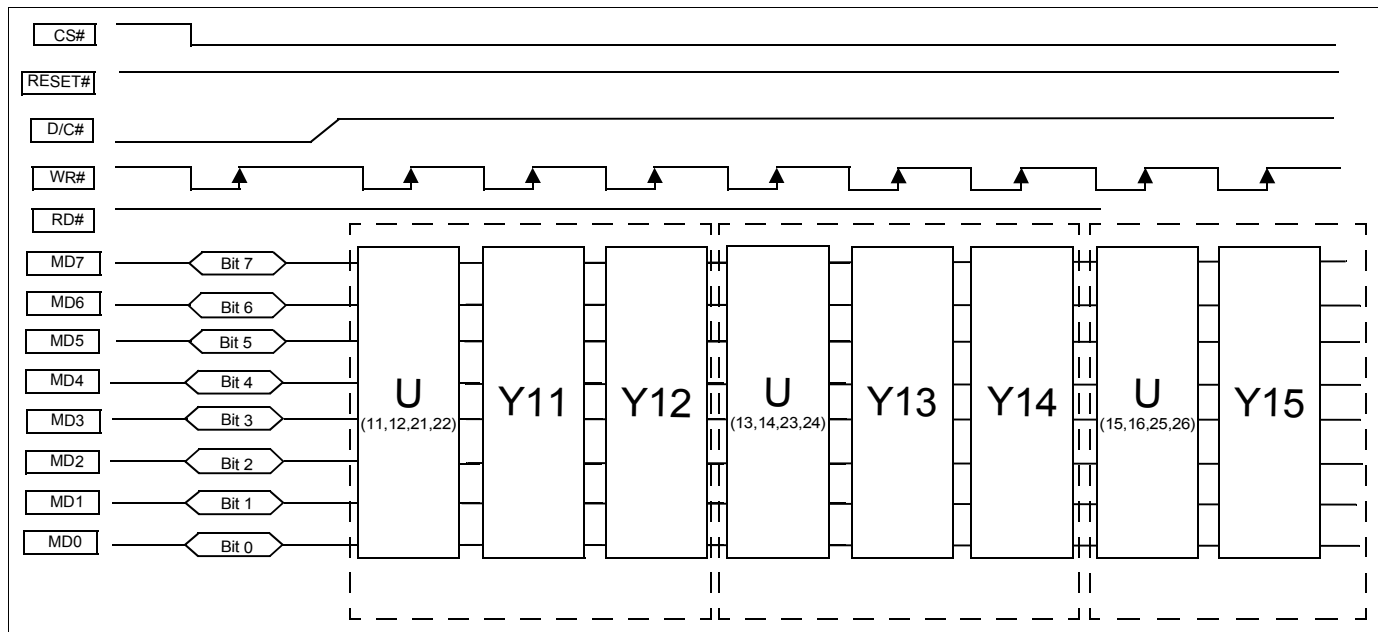
Figure 15-3: YUV 4:2:0 ODD Line with Intel 80, 8-bit Interface
