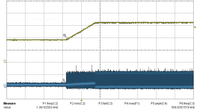
Fig. 8 - Pre-Bias Start-Up
