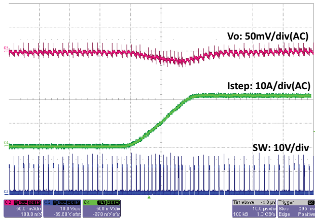
Fig. 51 - SiC450 Load Step, 20 A to 40 A, 1 A/ \mu\text{s} , t = 10\text{ }\mu\text{s}/\text{div}
