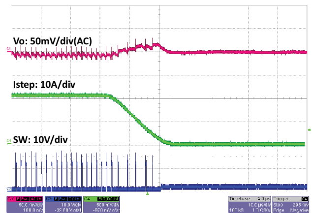
Fig. 56 - SiC450 Load Step, 20 A to 0 A, 1 A/ \mu\text{s} , t = 10\text{ }\mu\text{s}/\text{div} Skip Mode Enabled
