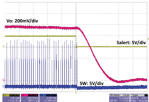
Fig. 16 - SiC453 UVP
