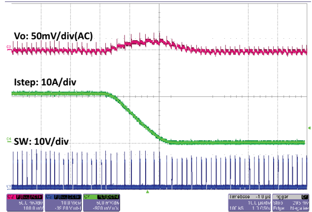
Fig. 54 - SiC450 Load Step, 20 A to 0 A, 1 A/ \mu\text{s} , t = 10\text{ }\mu\text{s}/\text{div}
