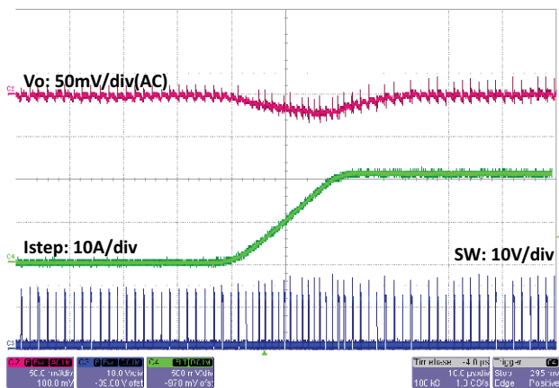
Fig. 53 - SiC450 Load Step, 0 A to 20 A, 1 A/ \mu\text{s} , t = 10\text{ }\mu\text{s}/\text{div}
