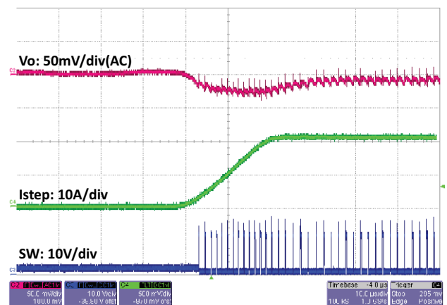
Fig. 55 - SiC450 Load Step, 0 A to 20 A, 1 A/ \mu\text{s} , t = 10\text{ }\mu\text{s}/\text{div} Skip Mode Enabled
