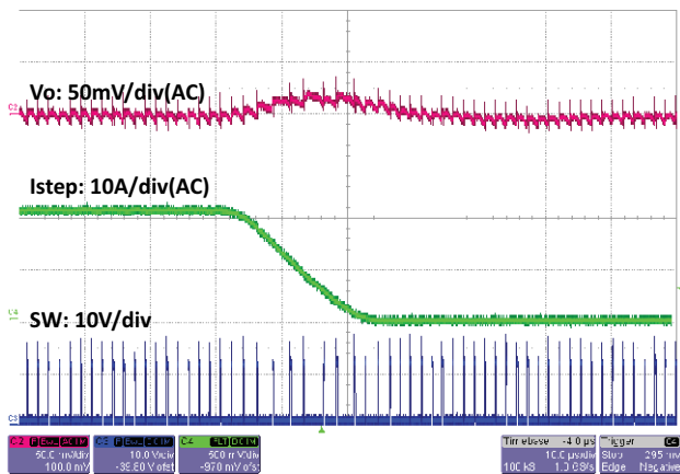
Fig. 52 - SiC450 Load Step, 40 A to 20 A, 10 A/ \mu\text{s} , t = 10\text{ }\mu\text{s}/\text{div}
