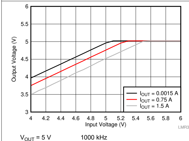
Figure 10-30. Overall Dropout Characteristic
