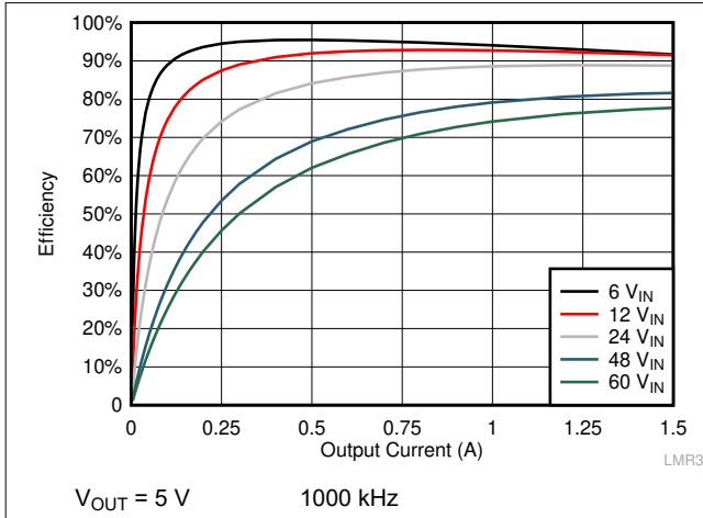
Figure 10-28. Efficiency
