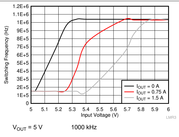
Figure 10-31. Frequency Dropout Characteristic
