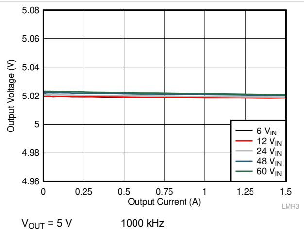
Figure 10-29. Load Regulation
