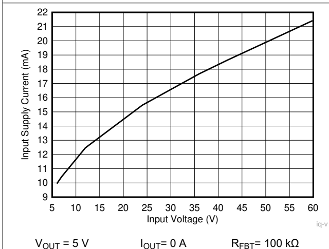
Figure 10-32. Input Supply Current
