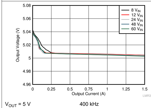
Figure 10-6. Load Regulation
