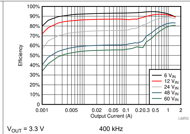
Figure 10-5. Efficiency
