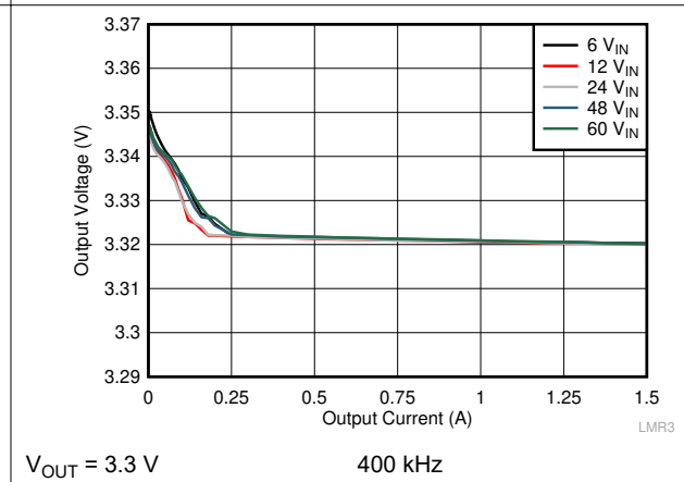
Figure 10-7. Load Regulation
