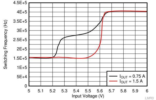
Figure 10-11. Frequency Dropout Characteristic
