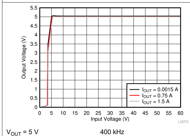
Figure 10-8. Line Regulation
