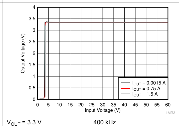
Figure 10-9. Line Regulation
