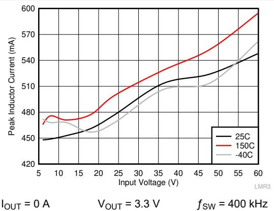
Figure 8-6. I PEAK-MIN
