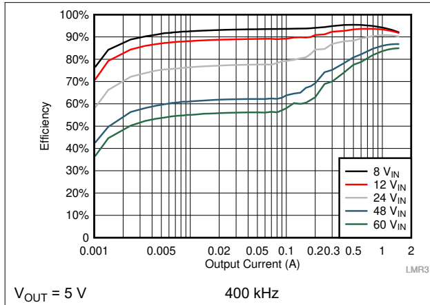
Figure 10-4. Efficiency
