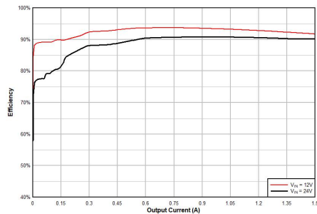
Efficiency
