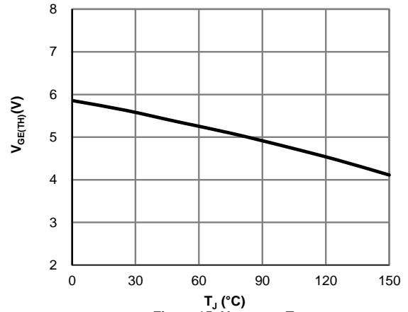
Figure 15: V_{GE(\text{TH})} vs. T_J
