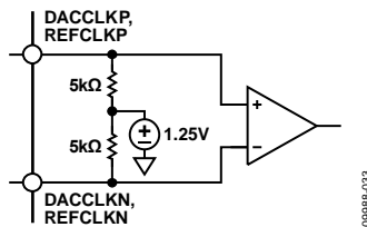
Figure 62. Clock Receiver Input Simplified Equivalent Circuit
