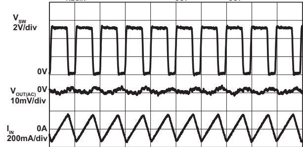
Time 400ns/div
