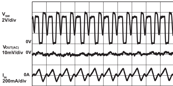
Time 400ns/div
